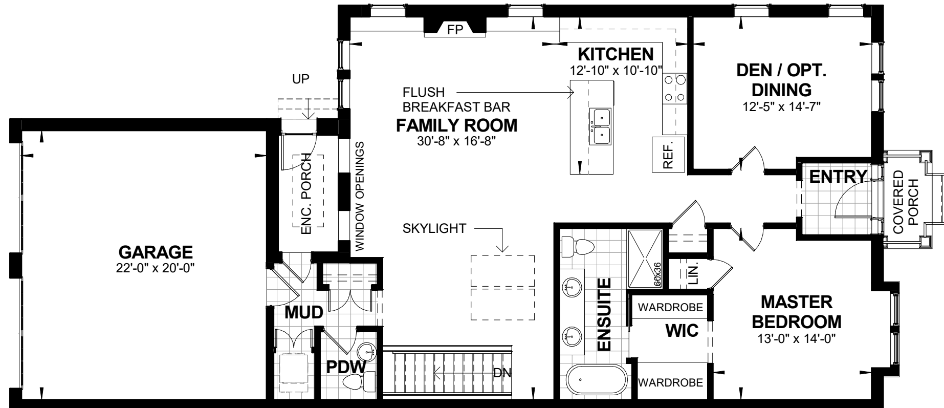
GROUND FLOOR PLAN - END OPT. FINISHED AREA 1519 sq. ft.
