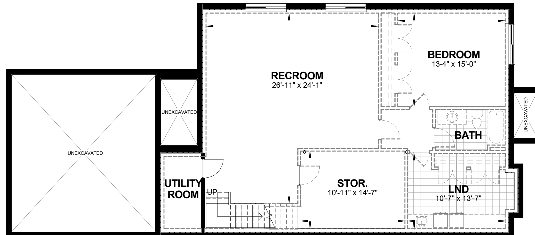
BASEMENT FLOOR PLAN - END OPT. FINISHED AREA 1219 sq. ft.
