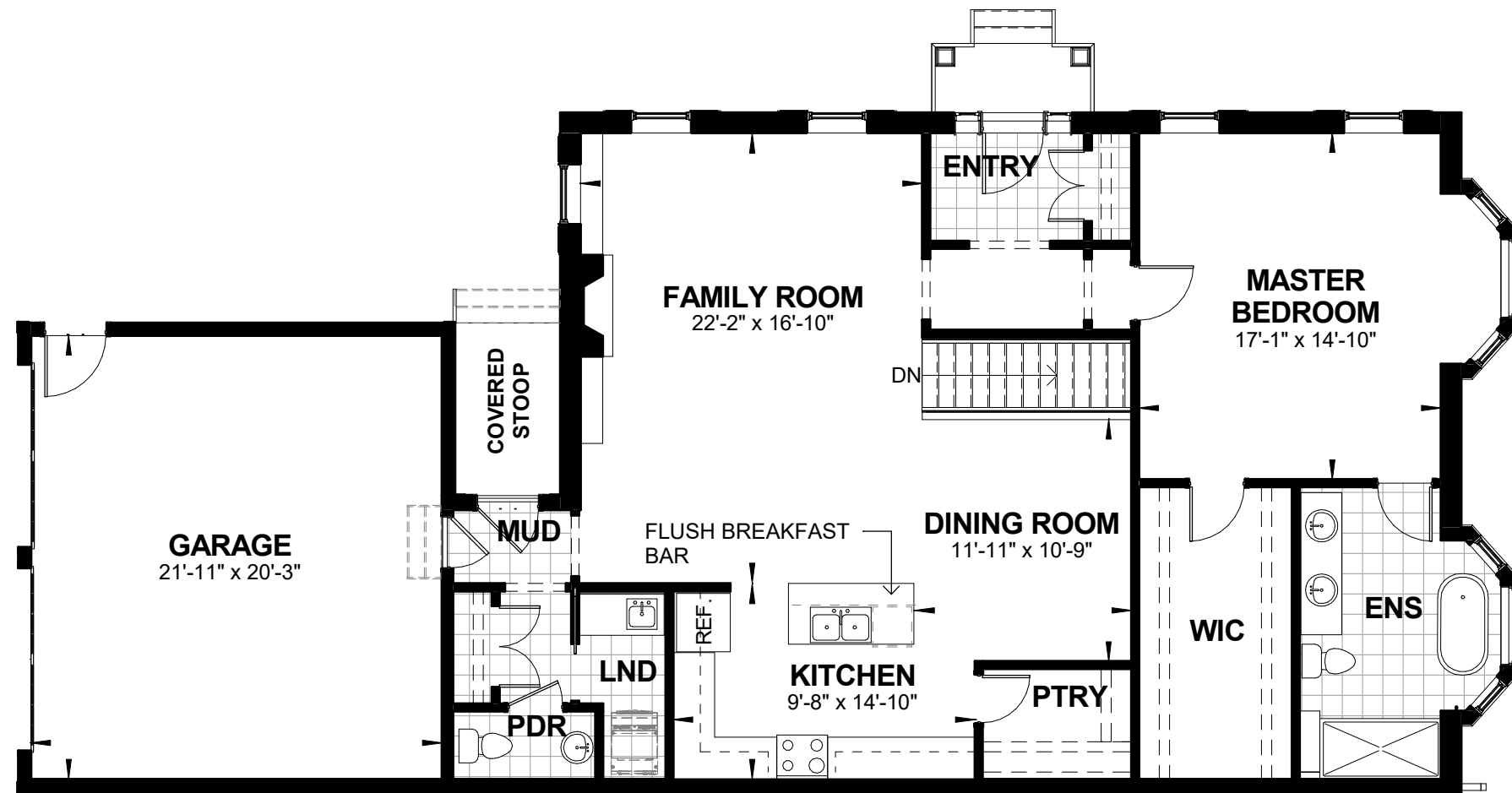
GROUND FLOOR PLAN - CORNER FINISHED AREA 1600 sq. ft.
