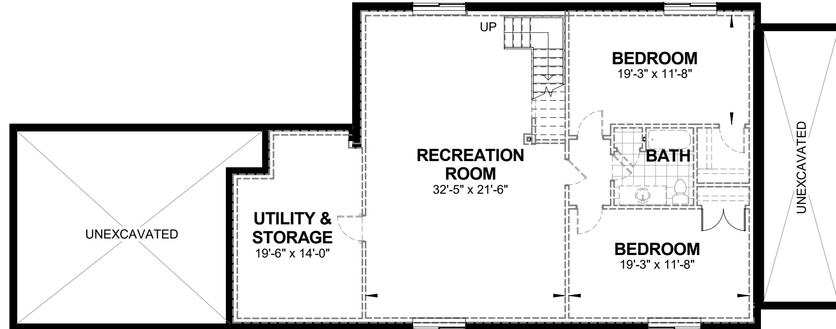
BASEMENT FLOOR PLAN OPT. FINISHED AREA 1441 sq. ft.
