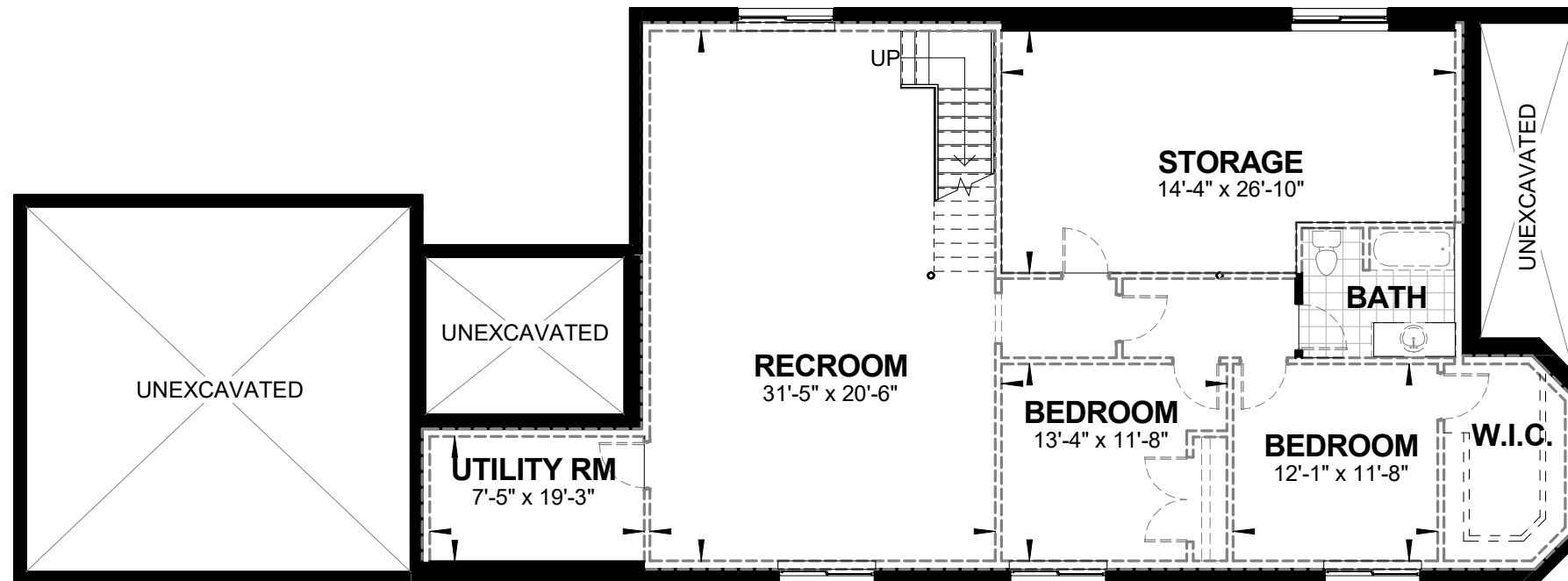
BASEMENT FLOOR PLAN OPT. FINISHED AREA 1307 sq. ft.
