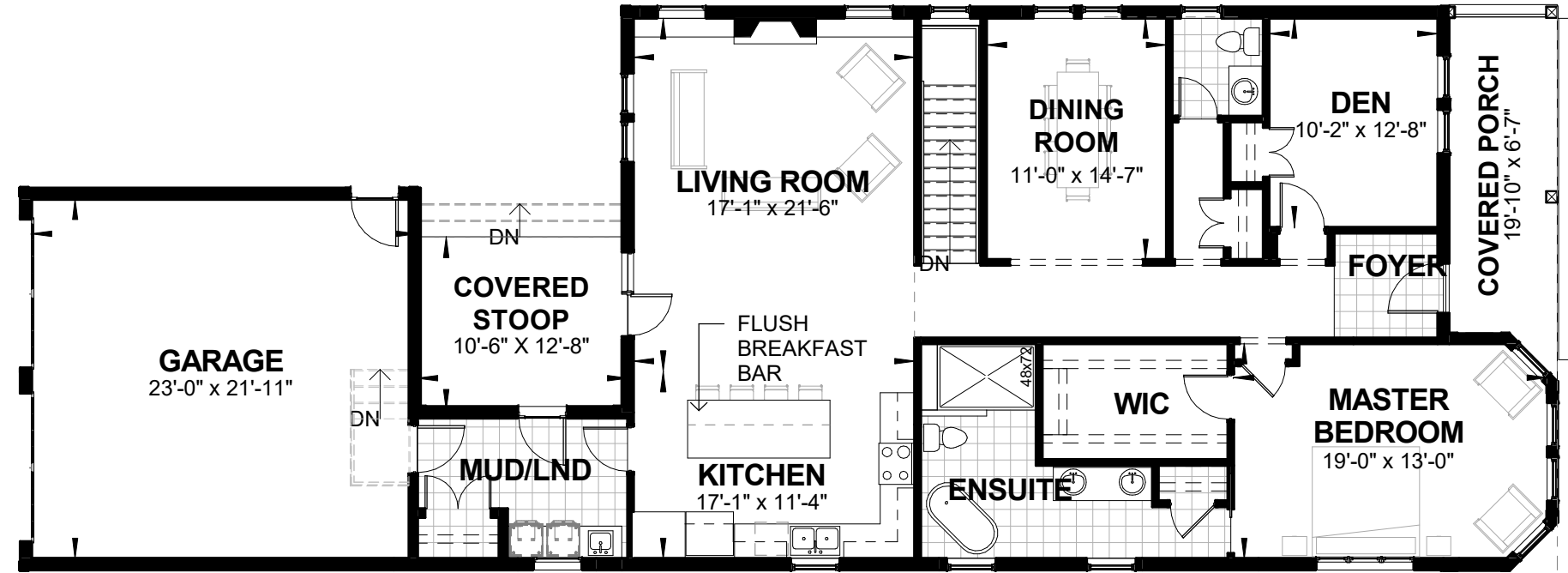
GROUND FLOOR PLAN FINISHED AREA 1931 sq. ft.
