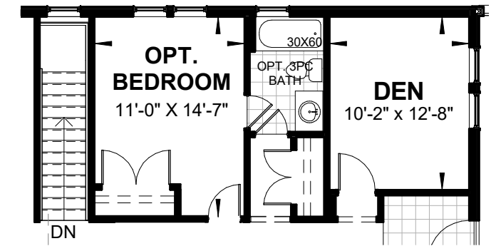
OPT. BEDROOM PLAN
