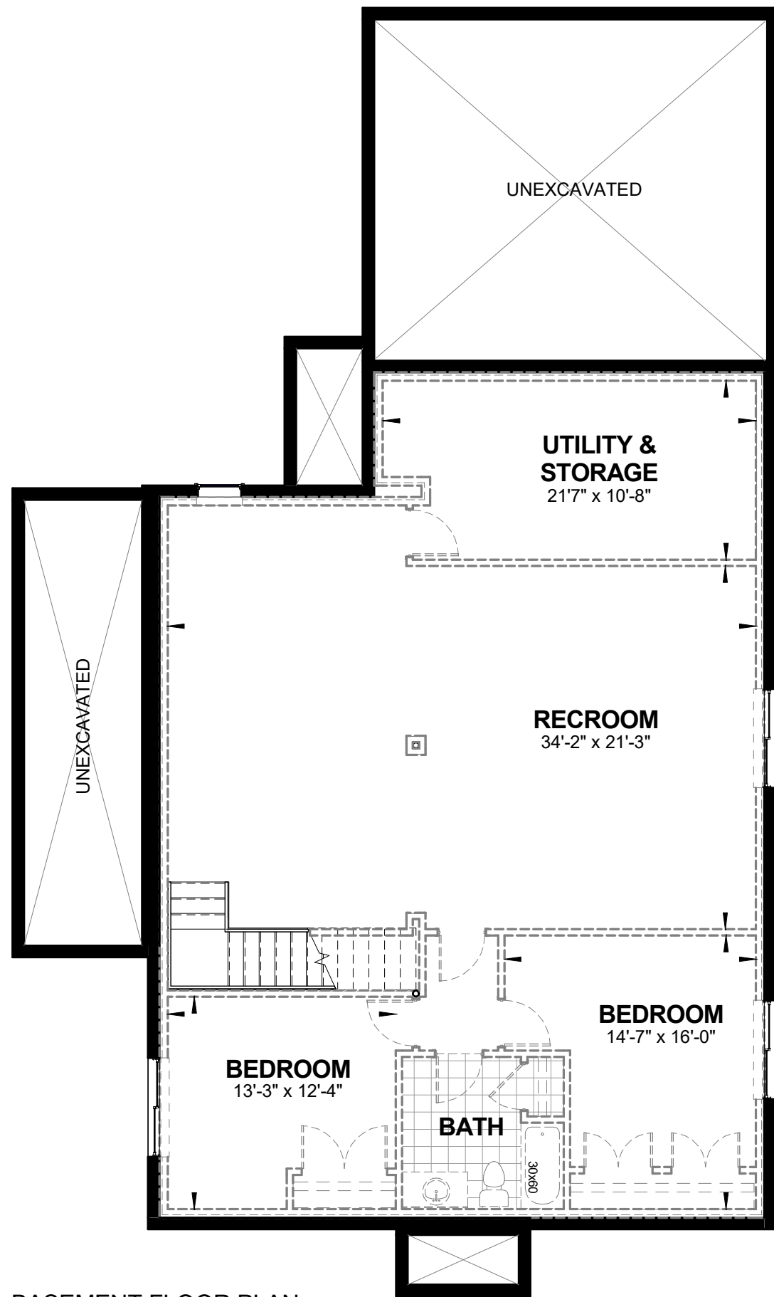
BASEMENT FLOOR PLAN OPT. FINISHED AREA 1459 sq. ft.
